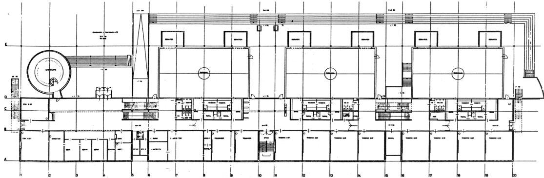
Gundriss
